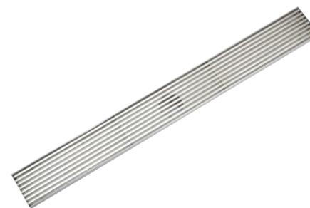
L910 (300~1200)x68x70mm SS304 DN:Ø45/50mm
