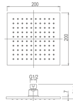
BSK083 WaterMark 200x200x7mm
